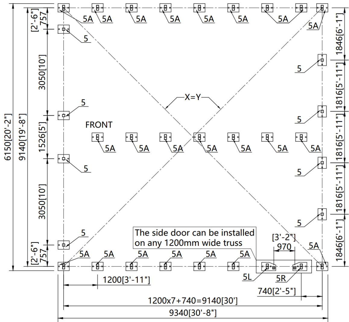
Installation diagram of expansion bolt.
